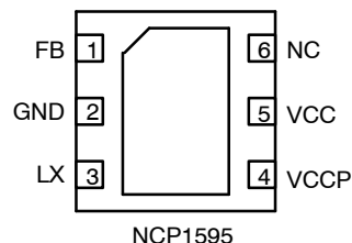
NCP1595
